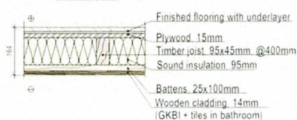
FF-2 / FLOOR
