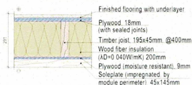
FF-1 / GROUND FLOOR
